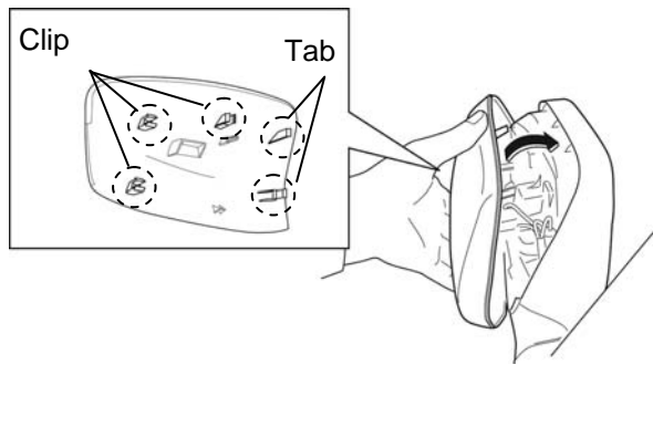
Backside of door mirror garnish
